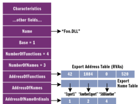
Figure 3 The IMAGE_EXPORT_DIRECTORY Structure
